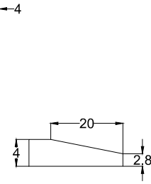
DETAIL X
