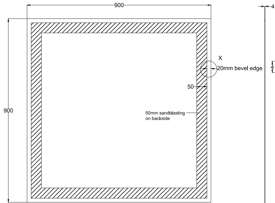
front view
